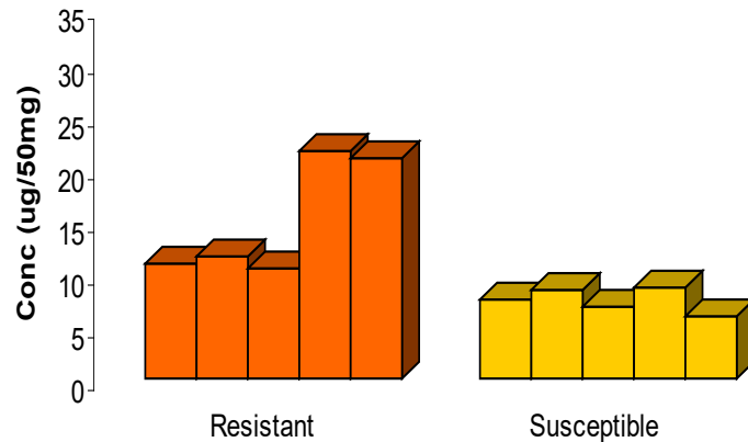
Chlorogenic acid
